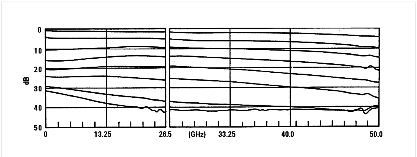
Figure 1. Typical Attenuation Characteristics
