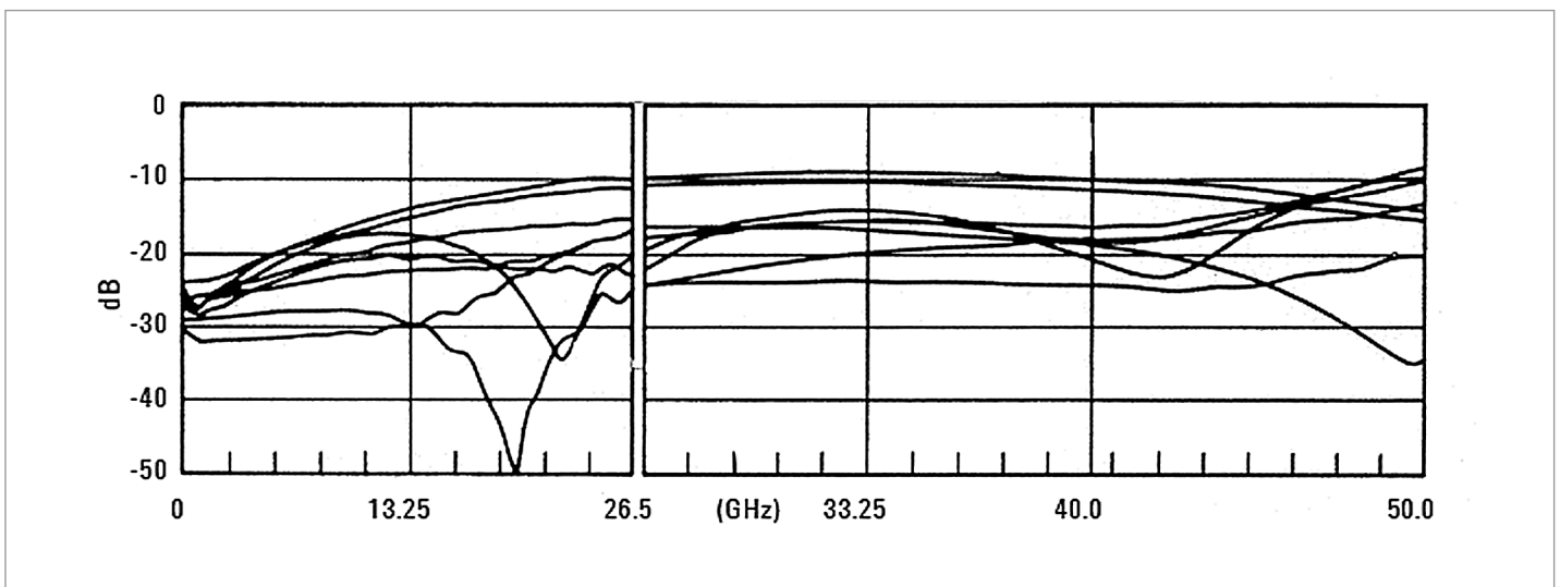
Figure 2. Typical Input and Output Return Loss
