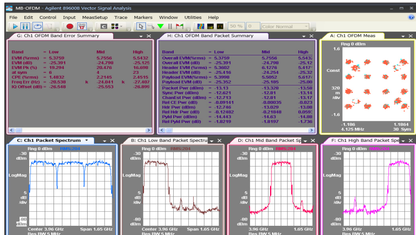
View the entire packet spectrum, or a single band. Choose from multiple summary tables to see EVM and power values per band. More detailed analysis per band is also available.
