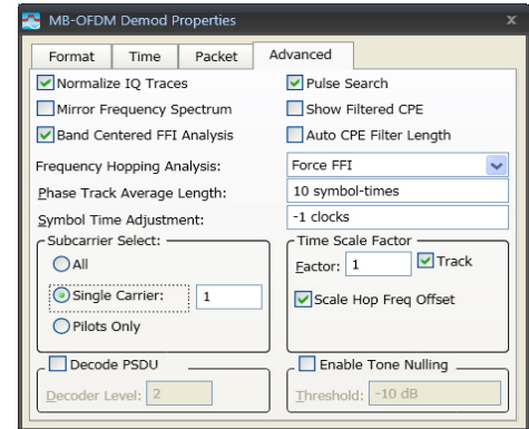
Option BHB simplifies measurement setup with automatic setting of many parameters. When you need to expose and investigate signal anomalies, the Advanced tab lets you access and adjust many detailed parameters.
