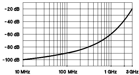
串扰 (50Ω)
