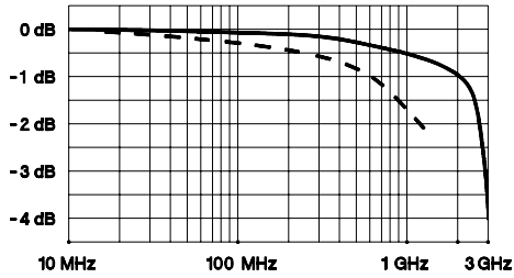
插入损耗 (50Ω)
