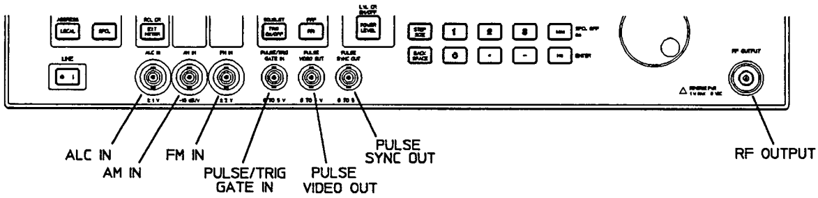
Figure 5-2. Synthesizer Connectors - Front Panel
