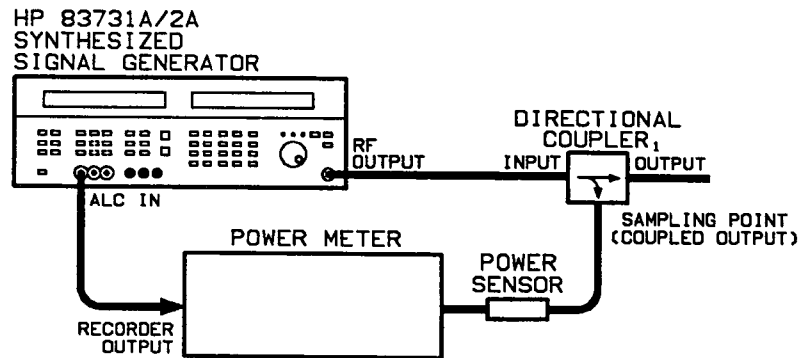
Figure 3-16. External Power Meter Leveling Setup
