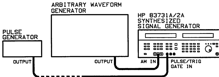
Figure 3-11. Antenna Scan Equipment Setup
