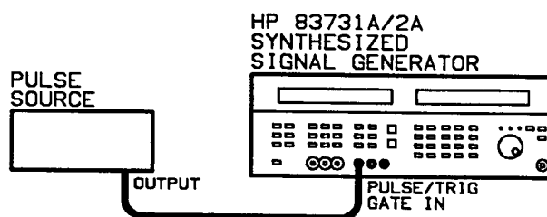
Figure 3-7. Doublet Pulse Equipment Setup
