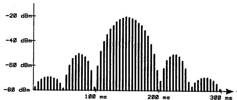
Figure 3-13. Example Modulated Antenna Scan Pattern
