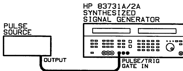
Figure 3-6. External Pulse Modulation Equipment Setup
