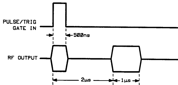
Figure 3-8. Doublet Pulse Mode Timing Example
