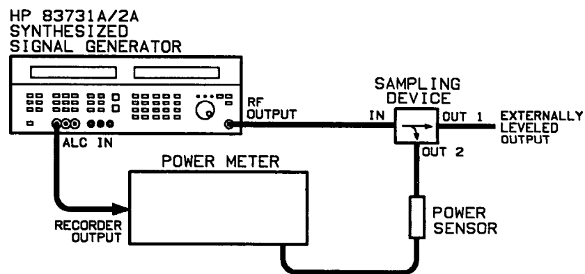
Figure 6-3. External Power Meter Leveling Setup
