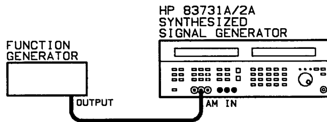
Figure 3-2. Log AM Equipment Setup
