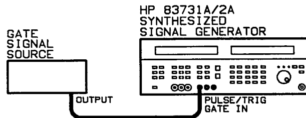
Figure 3-9. Gated Pulse Modulation Equipment Setup
