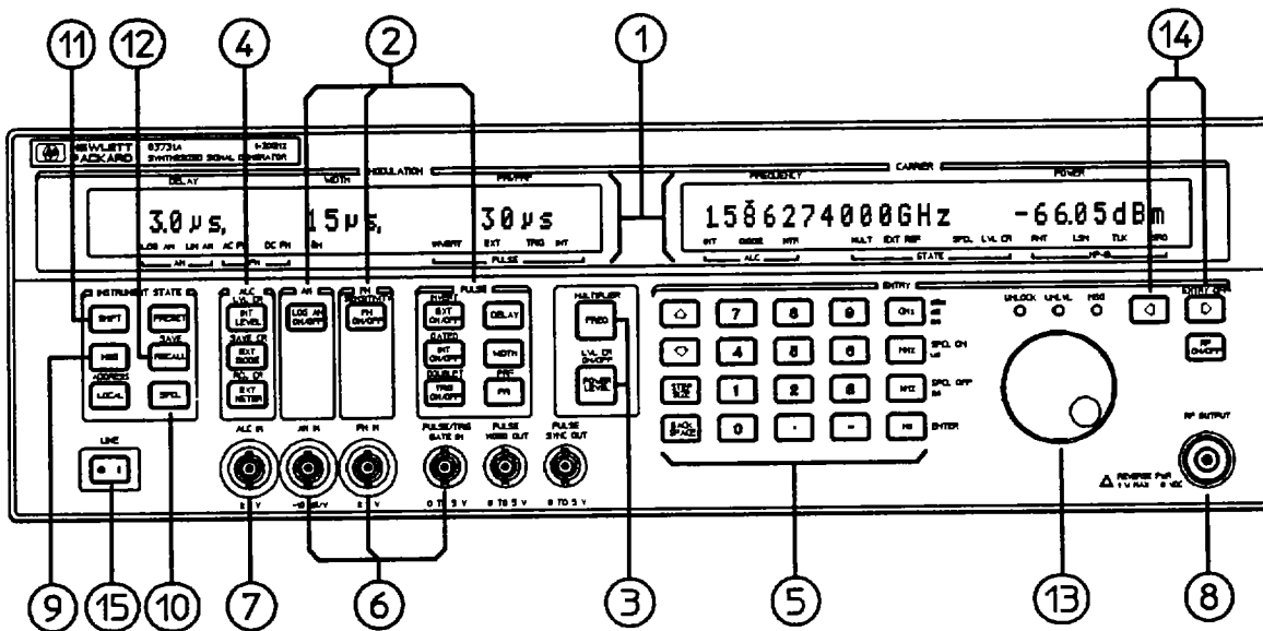
HP 83731A Synthesized Signal Generator
