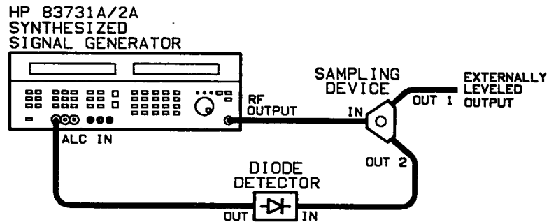
Figure 6-2. External Diode Detector Leveling Setup
