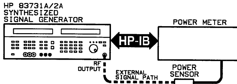
Figure 3-17. Level Correct Routine Equipment Setup
