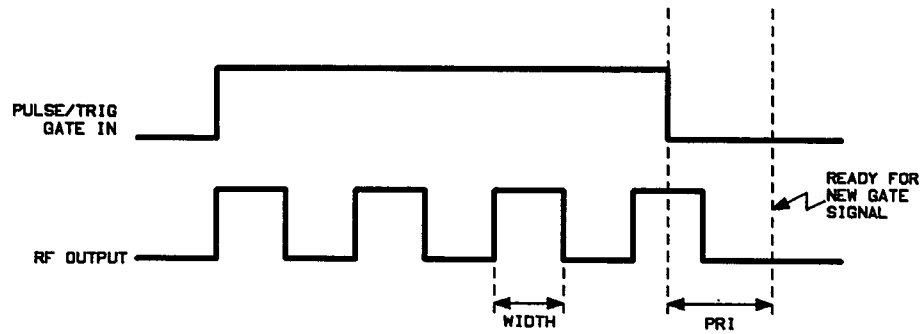
Figure 6-4. Internal Gated Pulse Mode Timing
