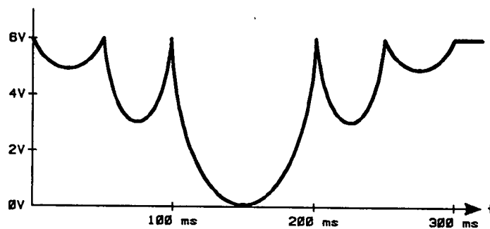
Figure 3-12. Example Antenna Scan Input
