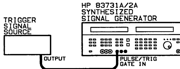
Figure 3-4. Externally Triggered Pulse Modulation Equipment Setup
