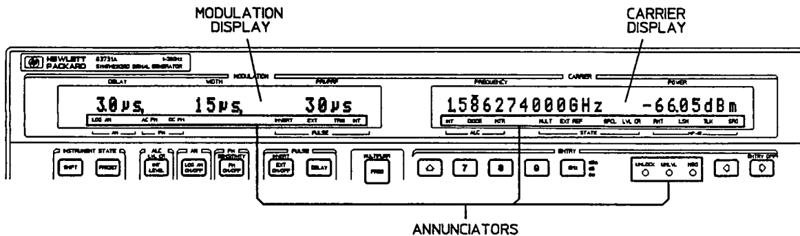
Figure 5-5. Synthesizer Display
