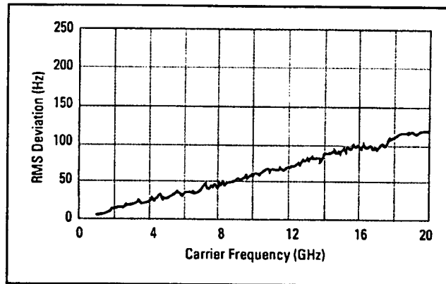
Typical residual FM measured in 50 Hz - 15 kHz bandwidth, CW mode, with high stability timebase (Option 1E5)
