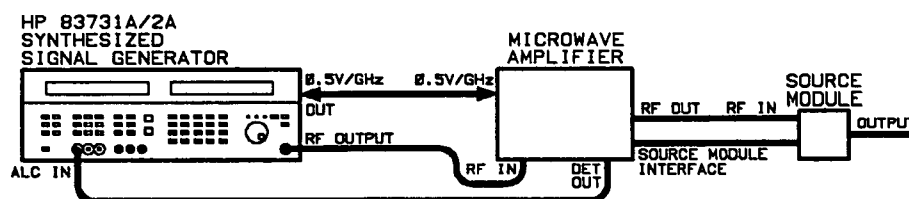
Figure 3-14. Millimeter-Wave Equipment Setup
