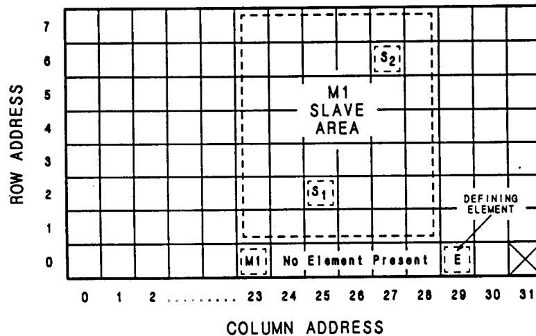
Figure 2-9. Master/Slave Addressing
