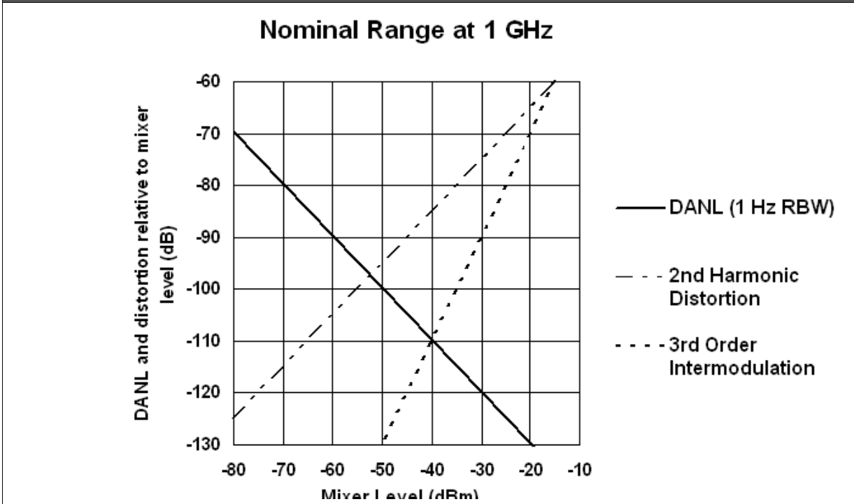
Nominal Dynamic Range at 1 GHz for Freq Option ≤ 526 [Plot]
